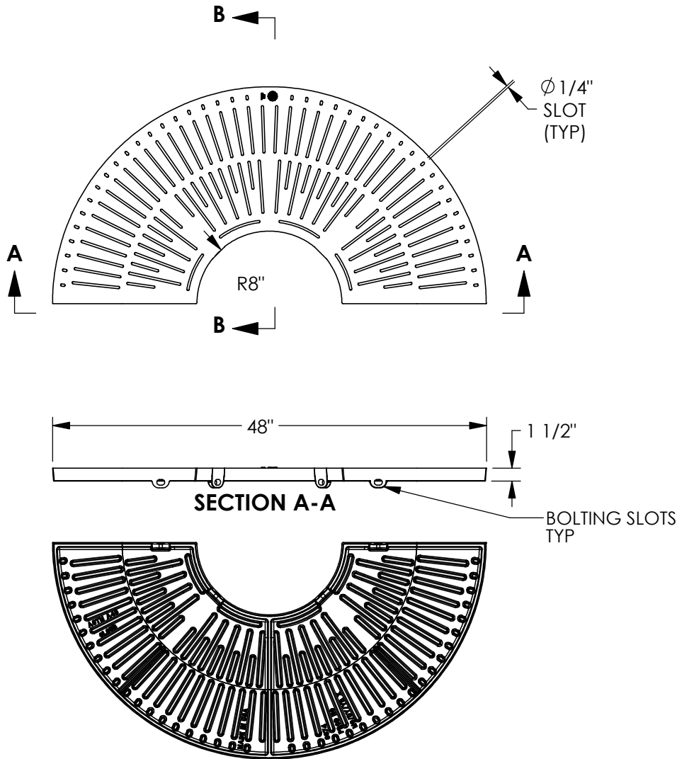
BOTTOM VIEW
